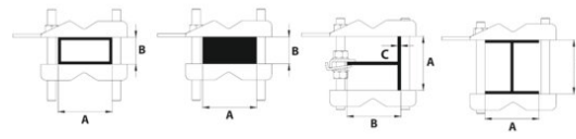
A-104mm / B-150mm / C-12mm
