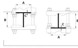
A-135mm / B-104mm / C-12mm
